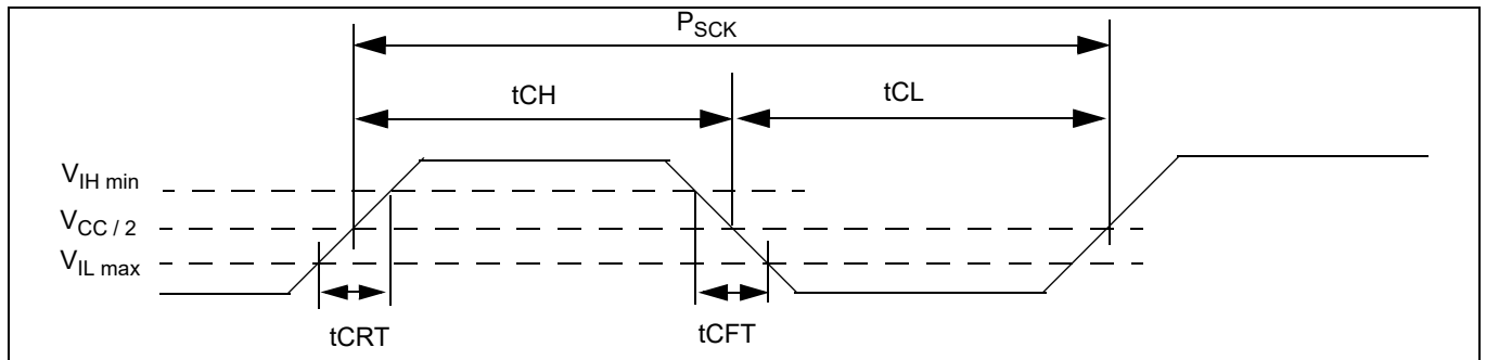
Figure 28 Clock timing
