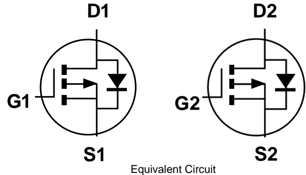
Equivalent Circuit
