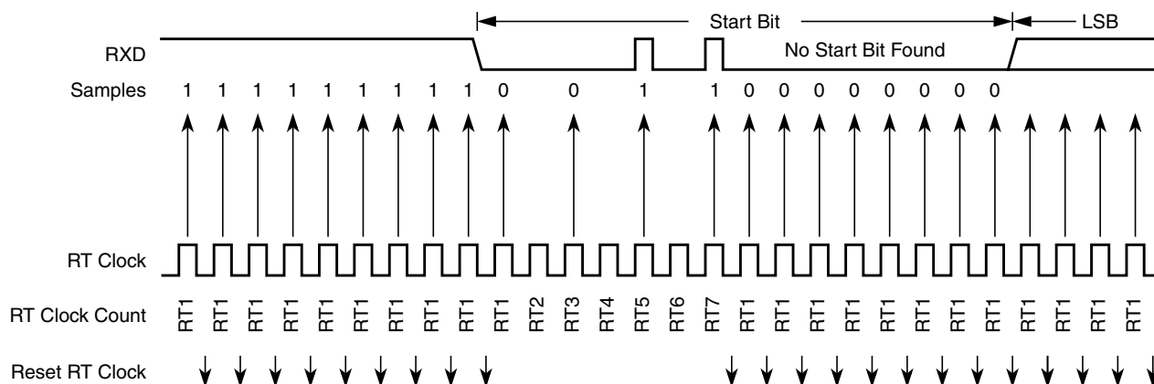
Figure 10-26. Start Bit Search Example 5
