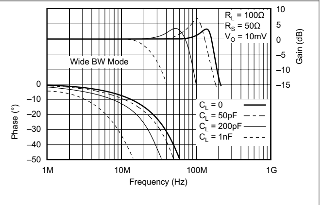
Figure 6-6. Gain and Phase vs Frequency vs Load Capacitance
