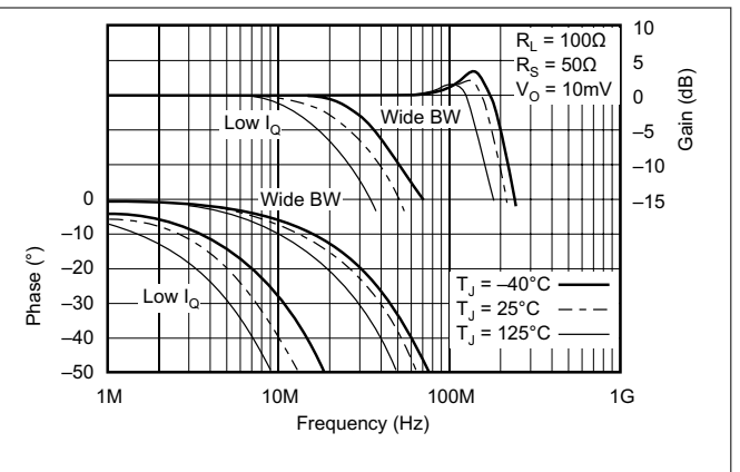
Figure 6-2. Gain and Phase vs Frequency vs Temperature
