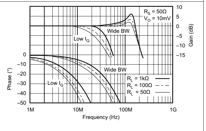
Figure 6-4. Gain and Phase vs Frequency vs Load Resistance
