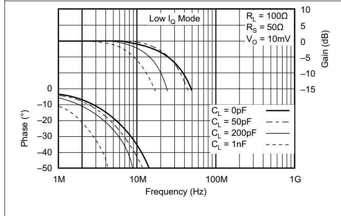
Figure 6-5. Gain and Phase vs Frequency vs Load Capacitance
