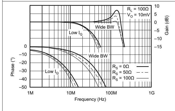
Figure 6-3. Gain and Phase vs Frequency vs Source Resistance
