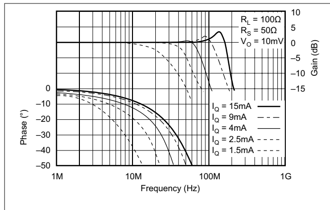
Figure 6-1. Gain and Phase vs Frequency vs Quiescent Current
