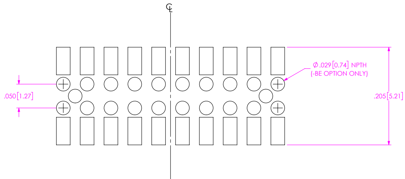
FIG 3 CLP-1XX-XX-XXX-D-BE-A SHOWN SAME AS FIG 1, DIFFERENT AS SHOWN ALL DIMENSIONS ARE SYMMETRIC ABOUT THE CENTERLINE
