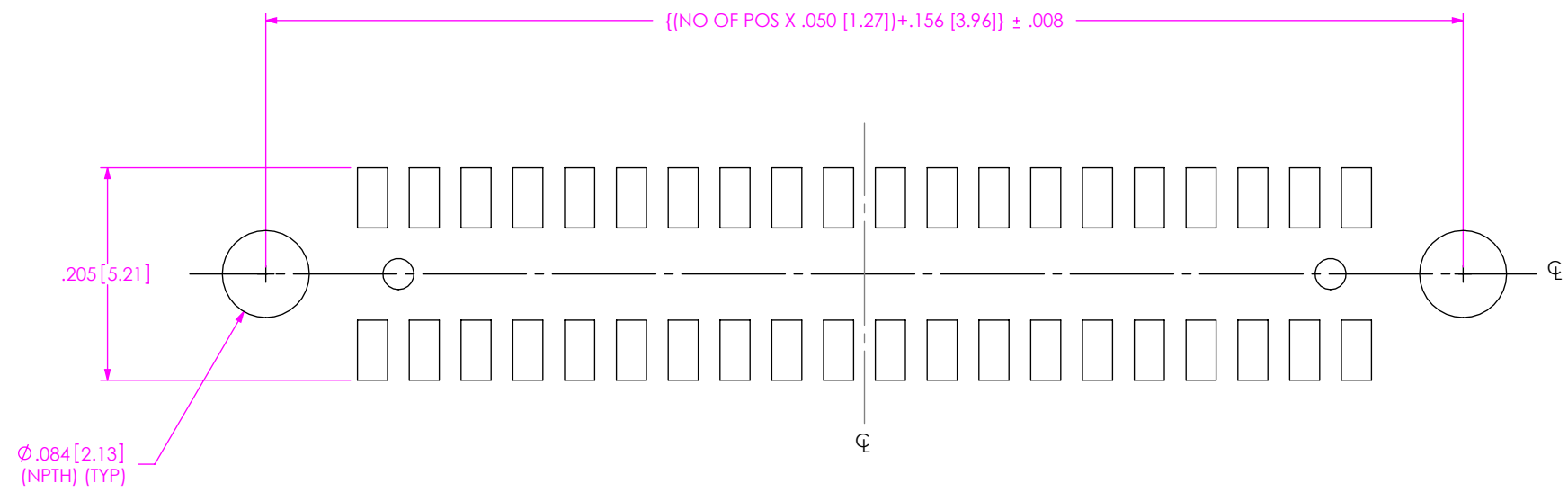
FIG 5 TO MATE CLP-1XX-XX-XXX-D-A WITH FTSH-EP / FW-EP SAME AS FIG 1, DIFFERENT AS SHOWN. ALL DIMENSIONS ARE SYMMETRIC ABOUT THE CENTERLINE.
