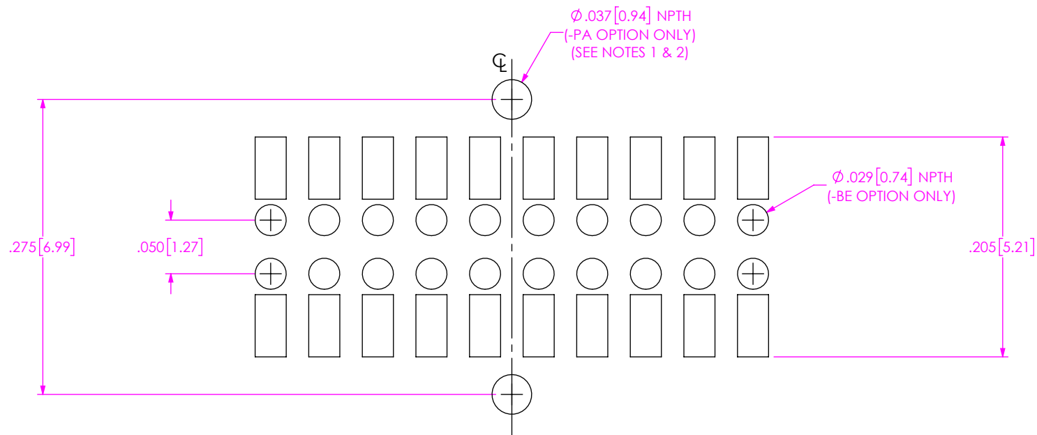
FIG 2 CLP-1XX-XX-XXX-D-BE-PA SHOWN SAME AS FIG 1, DIFFERENT AS SHOWN ALL DIMENSIONS ARE SYMMETRIC ABOUT THE CENTERLINE
