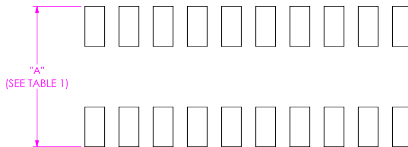
FIG 4 CLP-1XX-XX-XXX-D-XX SHOWN SAME AS FIG 1, DIFFERENT AS SHOWN ALL DIMENSIONS ARE SYMMETRIC ABOUT THE CENTERLINE
