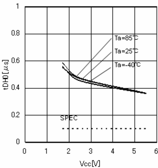
Figure 20. Output data hold time t_{DH1}
