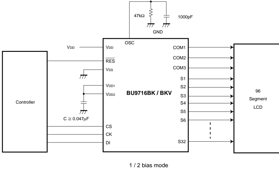
1 / 2 bias mode
