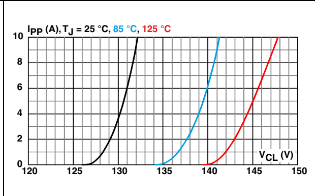
Figure 3. Clamping voltage versus peak pulse current - STRVS142X02F (typical values)
