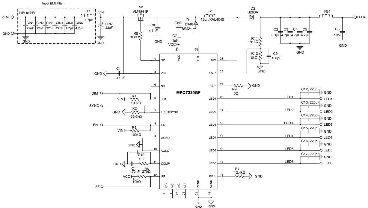
Figure 8: Typical Application Circuit for the TSSOP-28 Package with EMI Filters (I SET = 100mA, f sw = 410kHz)
