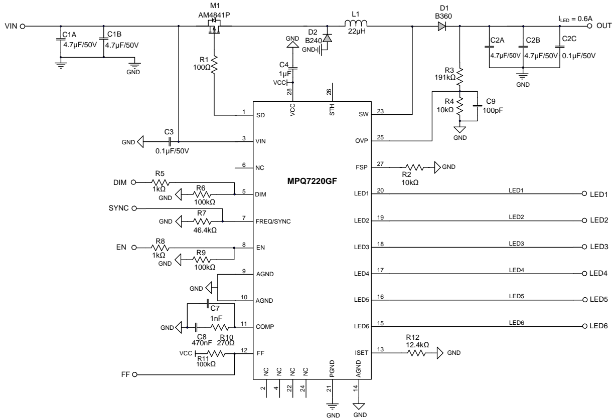
Figure 7: Typical Application Circuit for the TSSOP-28 Package (I SET = 100mA, f sw = 470kHz)
