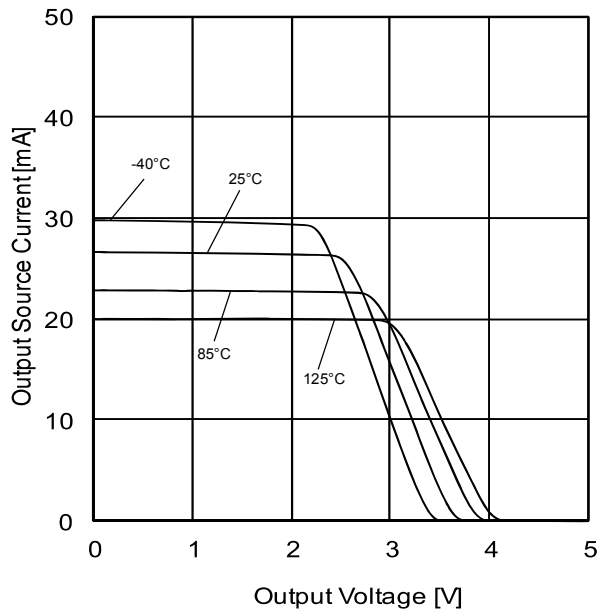
Figure 6. Output Source Current vs Output Voltage ( V_{CC}=5V )
