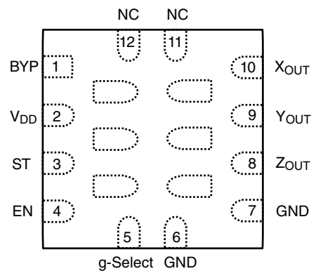
Figure 2. Pin locations
