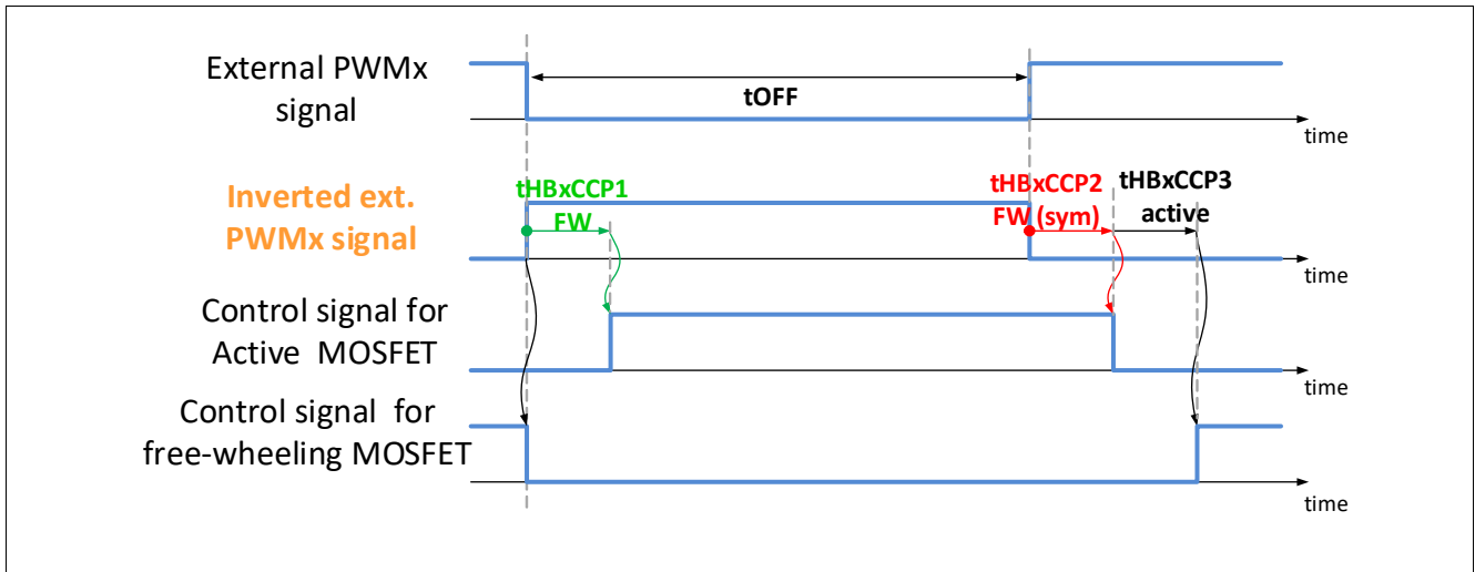
Figure 71 Internal signals for PWM operation - General case: t_{OFF} > t_{HBxCCP} + t_{HBxCCP} + t_{HBxCCP} , t_{ON} > t_{HBxCCP} + t_{HBxCCP} + t_{HBxCCP} , Motor operating as generator
