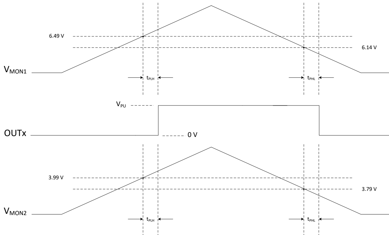
Figure 8-2. Overvoltage Detection
