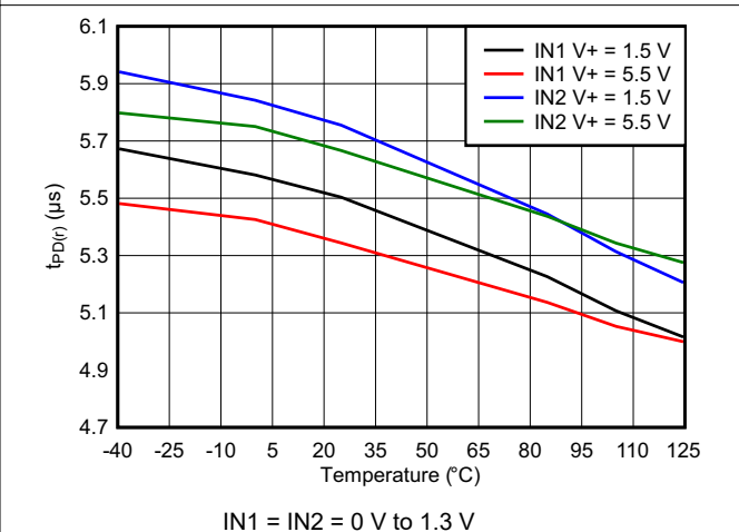
Figure 6-13. Propagation Delay from INx High to Output High
