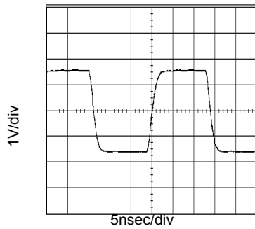
Fig.7 36MHz output waveform (VDD=3.3V, CL=15pF, Ta=25°C)
