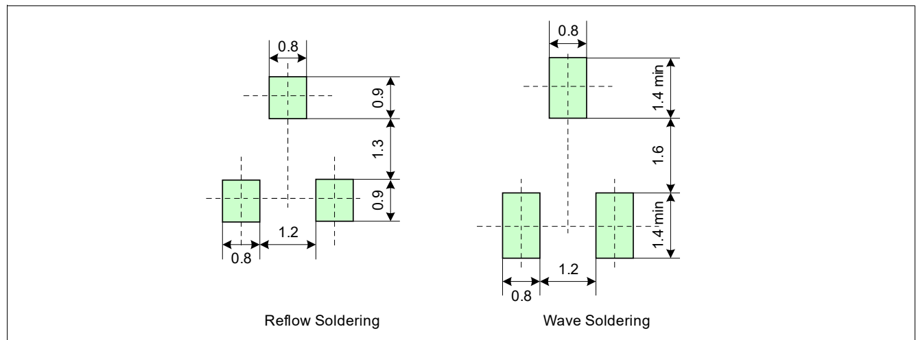
Figure 13 Footprint PG-SOT23-3-15
