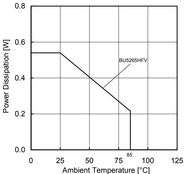
(c) BU5265HFV
