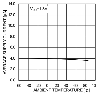
Fig.34 I DD - Ambient temperature
