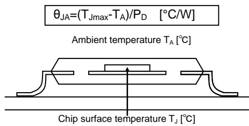
Figure 17. Thermal resistance
