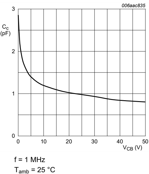
Fig. 9. PDTC143EQB-Q: Collector capacitance as a function of collector-base voltage; typical values
