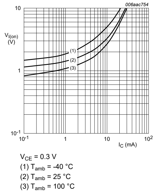
Fig. 25. PDTC144EQB-Q: On-state input voltage as a function of collector current; typical values
