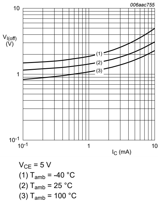
Fig. 26. PDTC144EQB-Q: Off-state input voltage as a function of collector current; typical values
