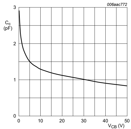
Fig. 15. PDTC114EQB-Q: Collector capacitance as a function of collector-base voltage; typical values
