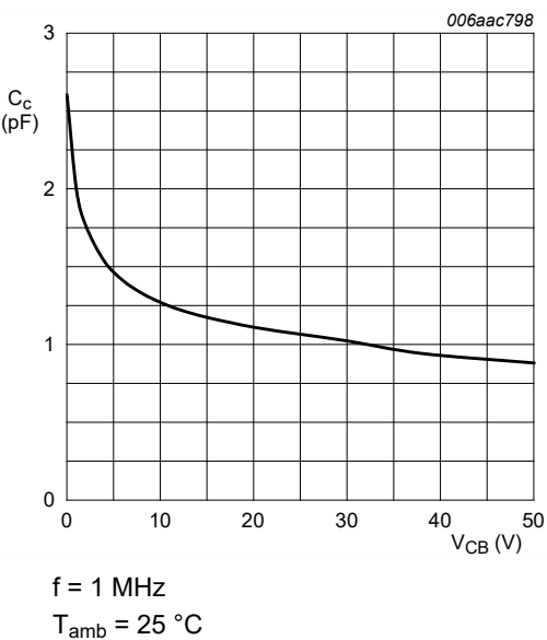
Fig. 21. PDTC124EQB-Q: Collector capacitance as a function of collector-base voltage; typical values
