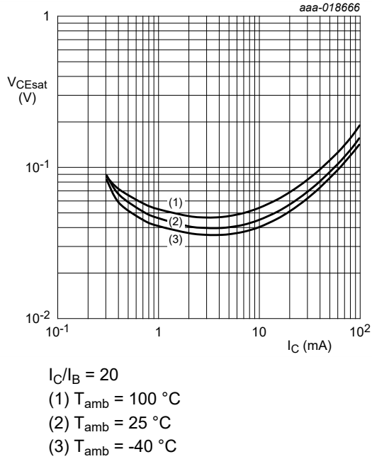
Fig. 24. PDTC144EQB-Q: Collector-emitter saturation voltage as a function of collector current; typical values
