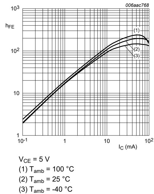
Fig. 10. PDTC114EQB-Q: DC current gain as a function of collector current; typical values
