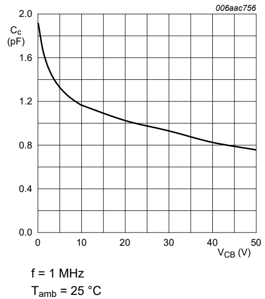
Fig. 27. PDTC144EQB-Q: Collector capacitance as a function of collector-base voltage; typical values
