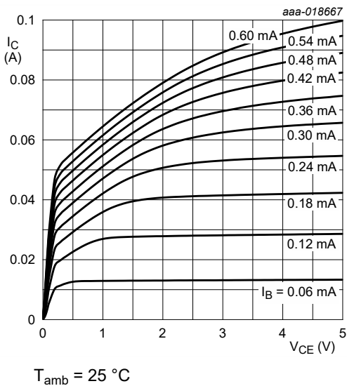
Fig. 23. PDTC144EQB-Q: Collector current as a function of collector-emitter voltage; typical values
