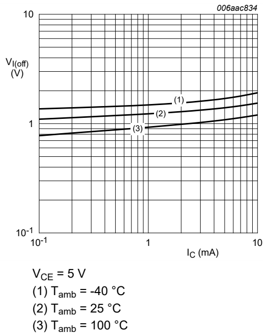
Fig. 8. PDTC143EQB-Q: Off-state input voltage as a function of collector current; typical values
