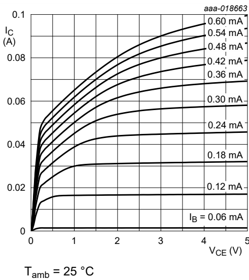
Fig. 11. PDTC114EQB-Q: Collector current as a function of collector-emitter voltage; typical values
