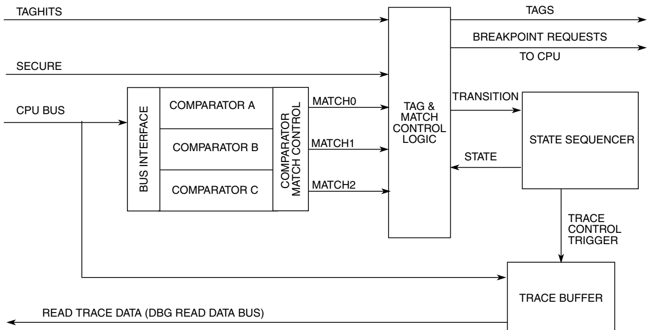
Figure 6-23. DBG Overview
