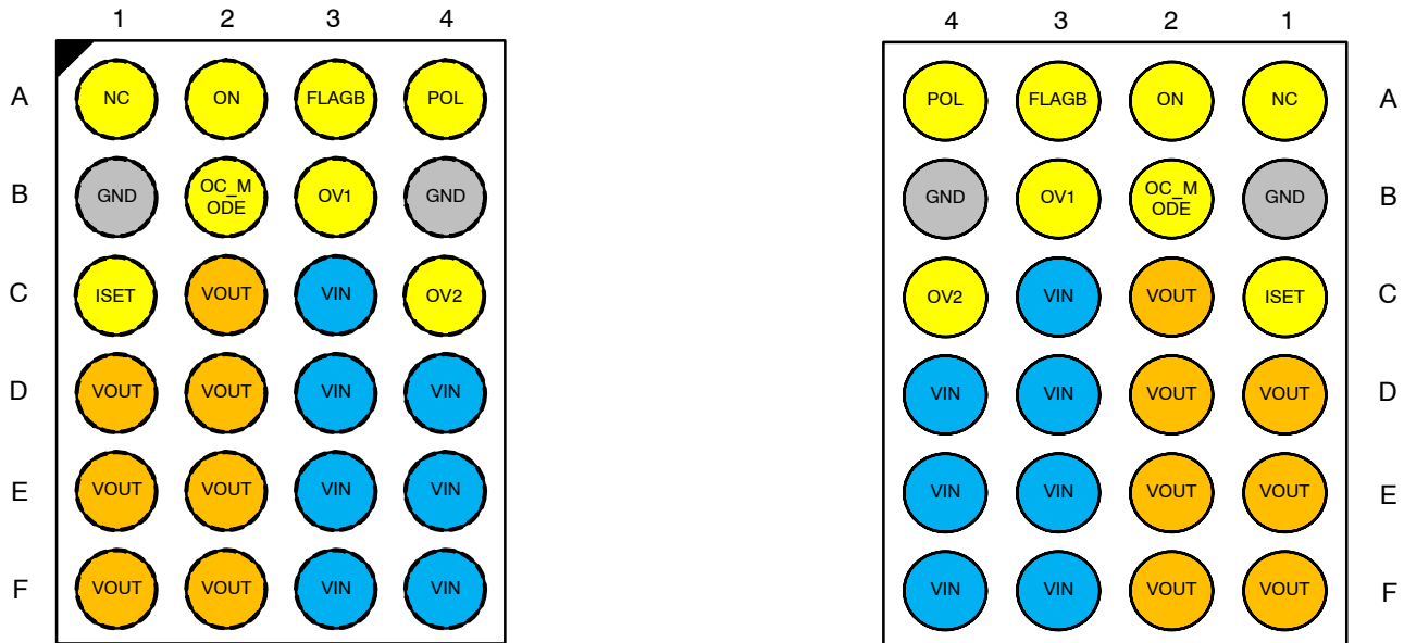
Figure 3. 24 Ball WL_CSP, 4 x 6 Array, 0.4 mm Pitch, 250 μm Ball
