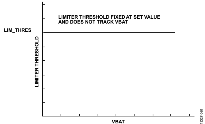
Figure 68. Limiter Fixed (LIM_EN = 0b01, VBAT_TRACK = 0b0)
