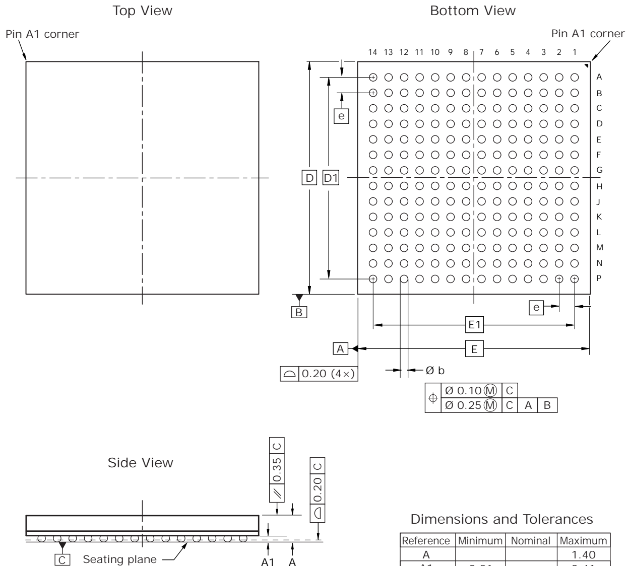
Figure 46 • Package Drawing
