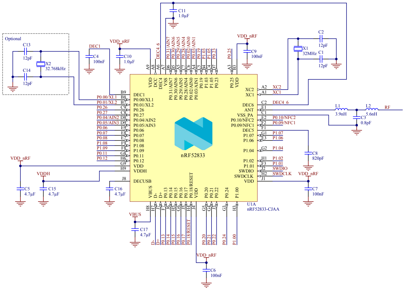
Figure 210: Circuit configuration no. 2 schematic for CJAA WLCSB
