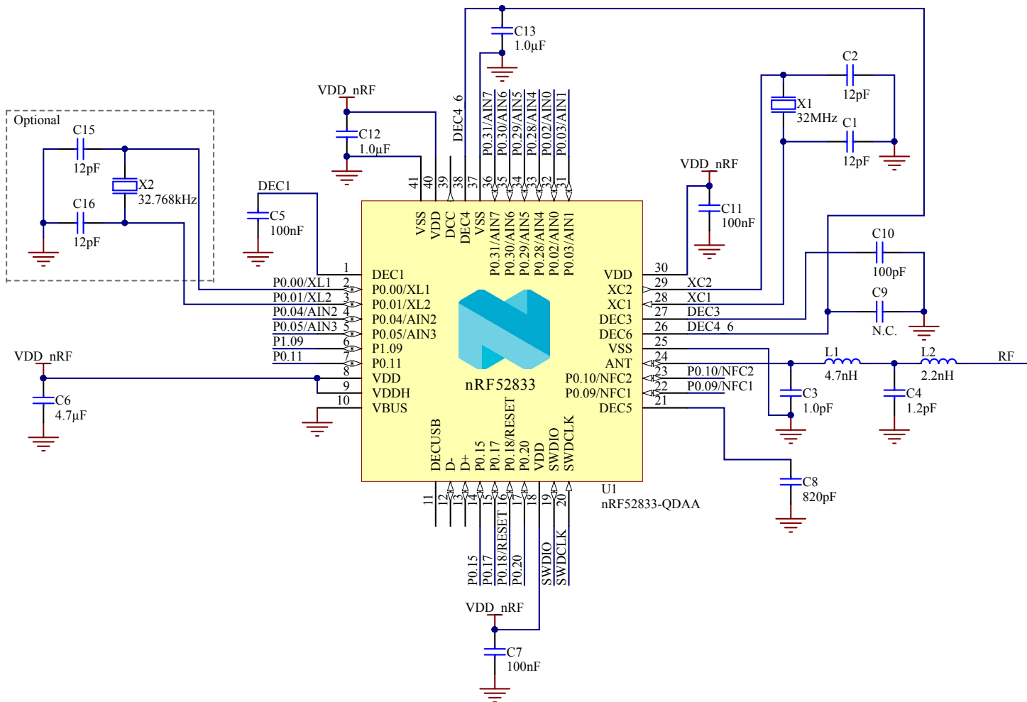
Figure 208: Circuit configuration no. 6 schematic for QDAA QFN40
