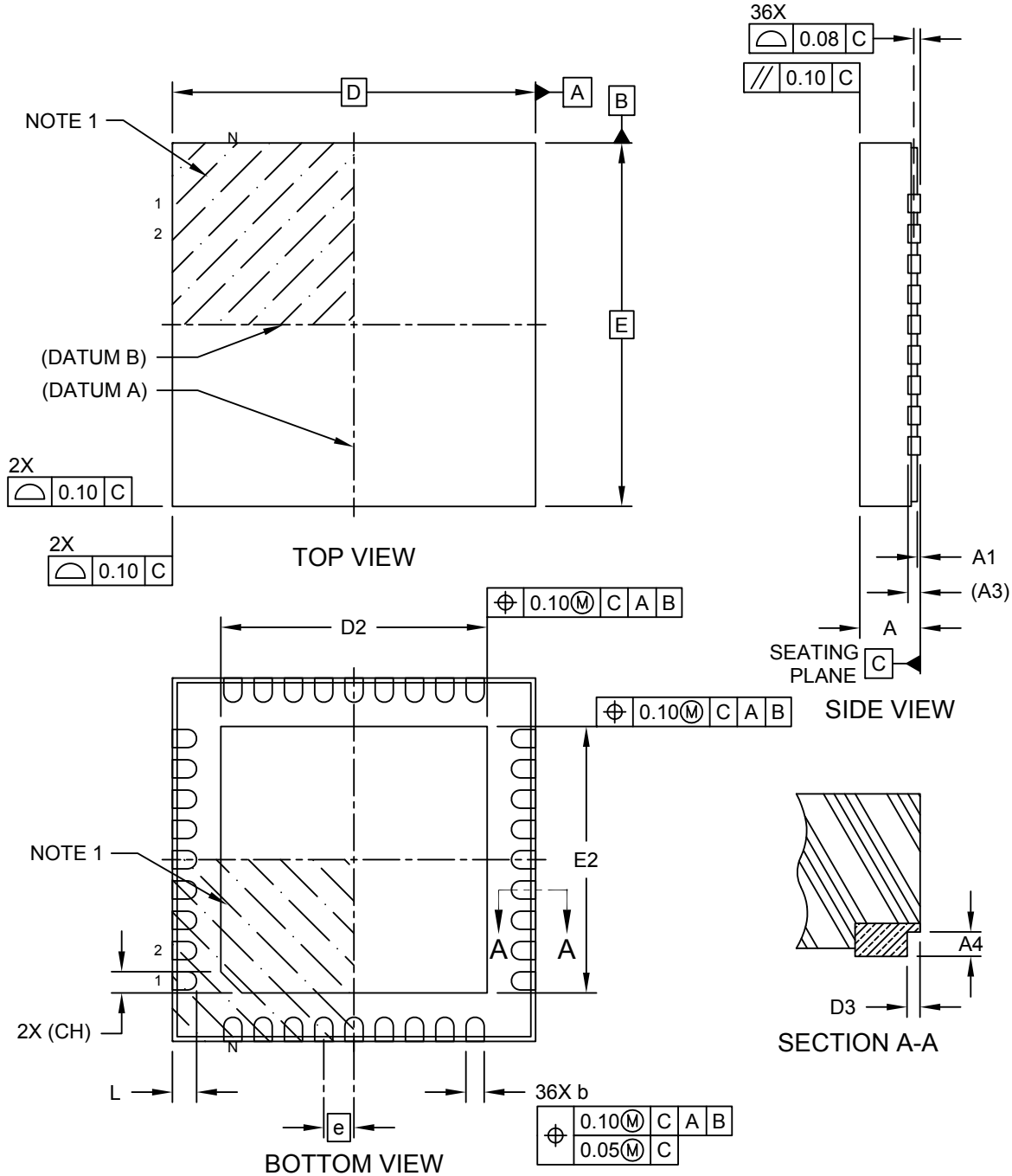
Microchip Technology Drawing C04-501 Rev B Sheet 1 of 2
