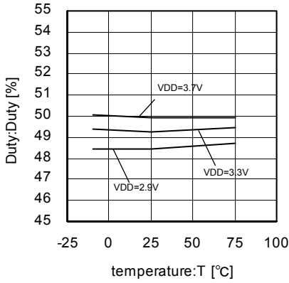
Fig.59 54MHz Duty temperature characteristics
