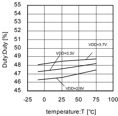
Fig.64 67.5MHz Duty temperature characteristics
