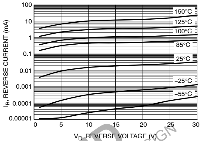
Figure 6. Leakage Current
