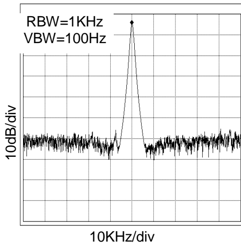
Figure 15. 48MHz Spectrum (At V_{DD}=3.3V and C_L=15pF )
