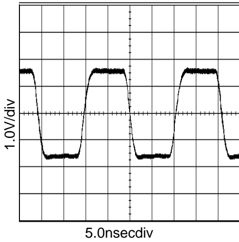
Figure 13. 48MHz Output Wave (At V_{DD}=3.3V and C_L=15pF )
