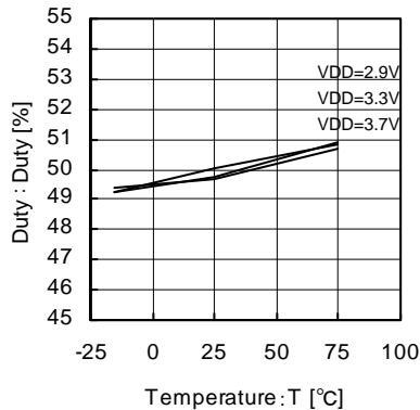
Fig.52 27MHz BUFFER Temperature-Duty
