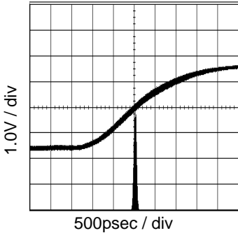
Fig.7 36.864MHz Period-Jitter VDD=3.3V,CL=32pF
