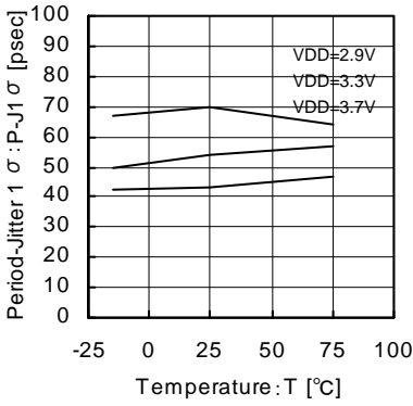
Fig.40 18.432MHz Temperature - Period-Jitter 1 \sigma
