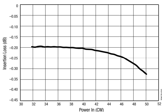
Figure 10. Insertion Loss vs CW Input Power (ANT to TX Port, f = 2.4 GHz)
