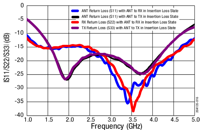
Figure 16. Return Loss vs Frequency
