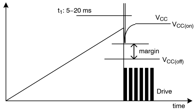
Figure 40. Startup Process for NCP112x
