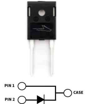
Package Types: TO-247-2 Marking: C4D15120
