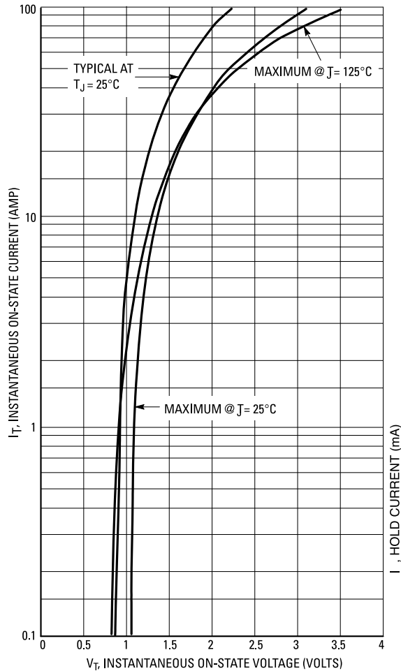
Figure 3. On-State Characteristics
