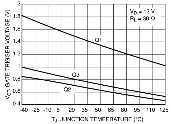
Figure 7. Typical Gate Trigger Voltage Variation
