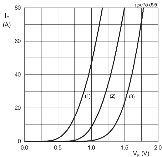
(1) T_j = 150\text{ °C} ; typical values (2) T_j = 150\text{ °C} ; maximum values (3) T_j = 25\text{ °C} ; maximum values V_o = 1.147\text{ V}; R_s = 0.0043\ \Omega
