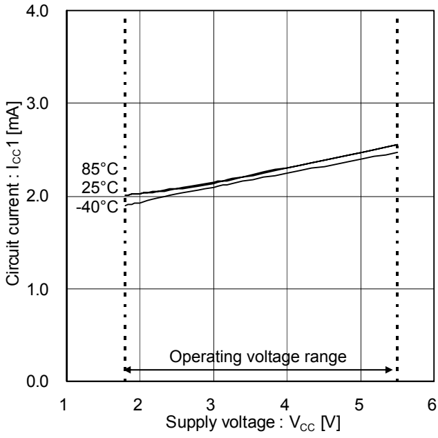
Figure 3. Circuit Current 1
