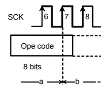
Figure 48. WREN/WRDI cancel valid timing
