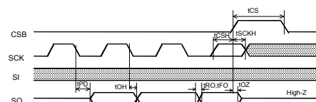
Figure 2-(b). Input / Output timing
