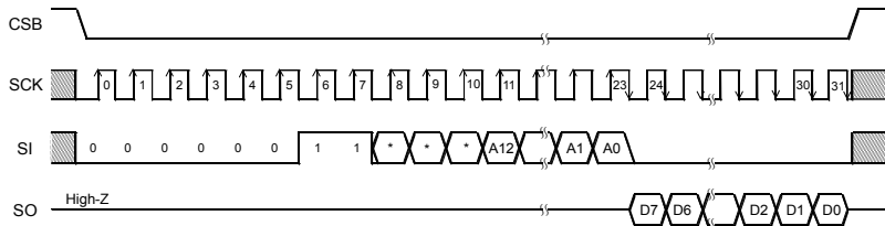
Figure 39. Read command
