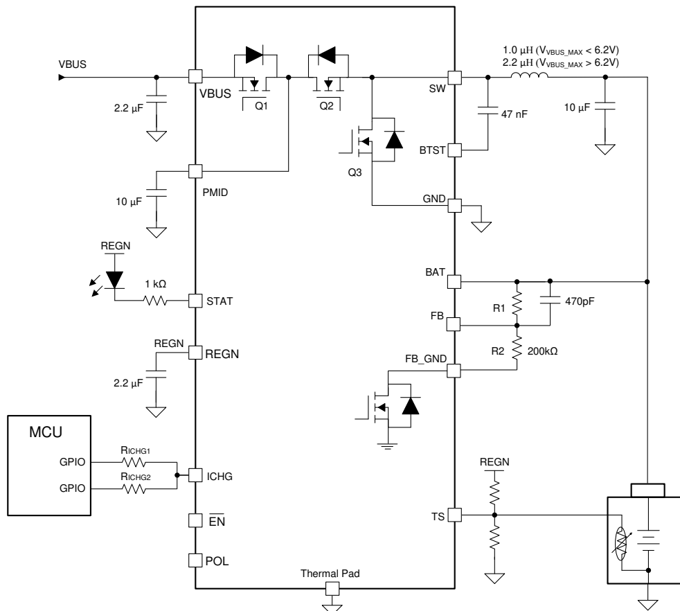
Figure 10-9. Typical Application with MCU Programmed Charge Current (1-µH inductor is recommended if maximum input voltage V_{\text{VBUS\_MAX}} < 6.2\text{V} ; 2.2-µH inductor is recommended if maximum input voltage V_{\text{VBUS\_MAX}} > 6.2\text{V} )
