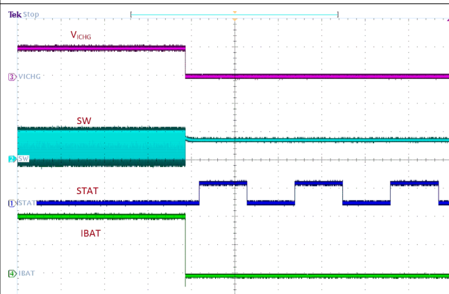
Figure 9-3. Charge Cycle with Battery Simulator
