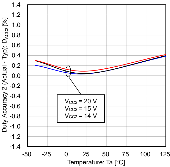
Figure 35. Duty Accuracy 2 (Actual - Typ) vs Temperature
