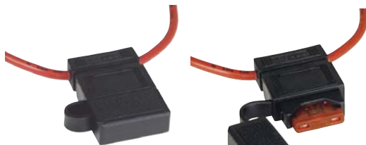
BF351 25A- 12AWG wire water resistant ATP/ATC/ATO fuses
