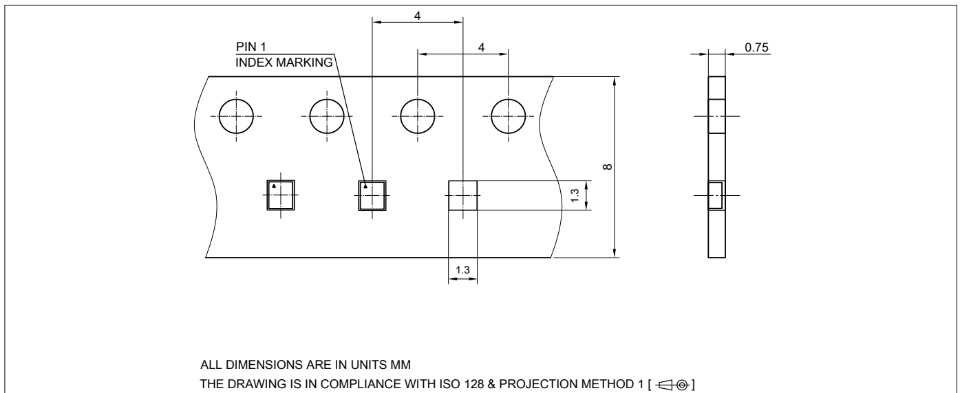
Figure 6: Carrier Tape
