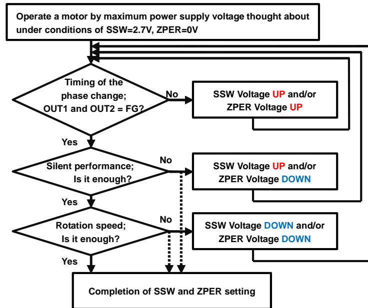
Figure 41. Flow of Setting of SSW and ZPER Terminal
