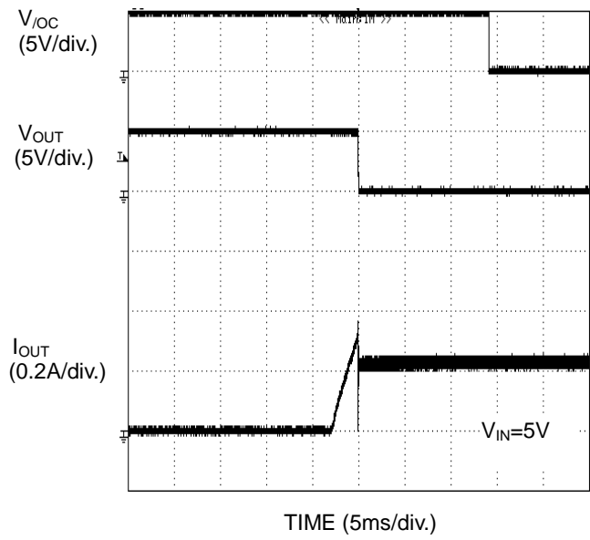
Figure 32. Over-Current Response
