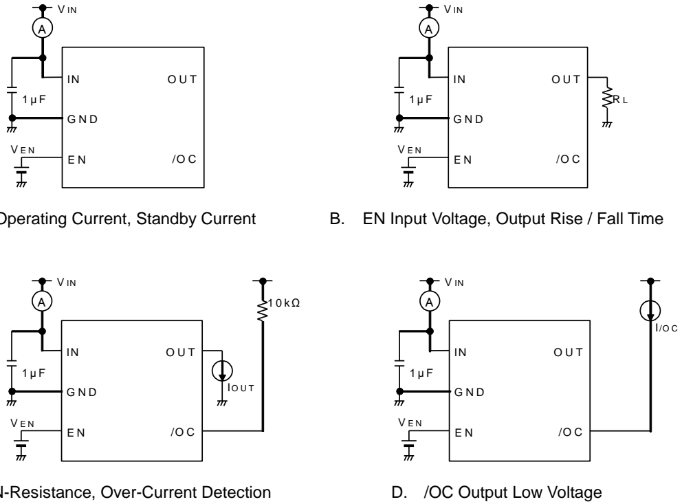
Figure 1. Measurement Circuit
