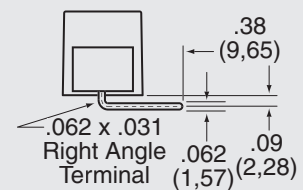
7 – Right Angle Printed Circuit Pin
