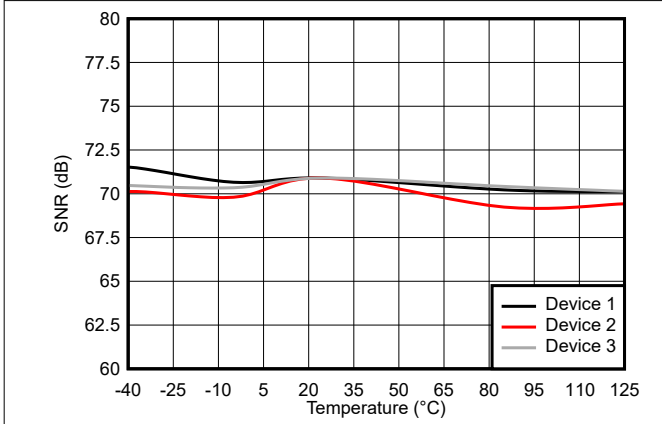
Figure 6-23. Signal-to-Noise Ratio vs Temperature
