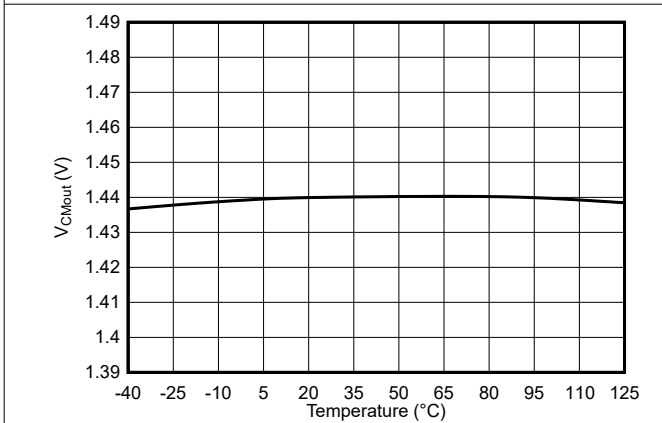
Figure 6-27. Output Common-Mode Voltage vs Temperature
