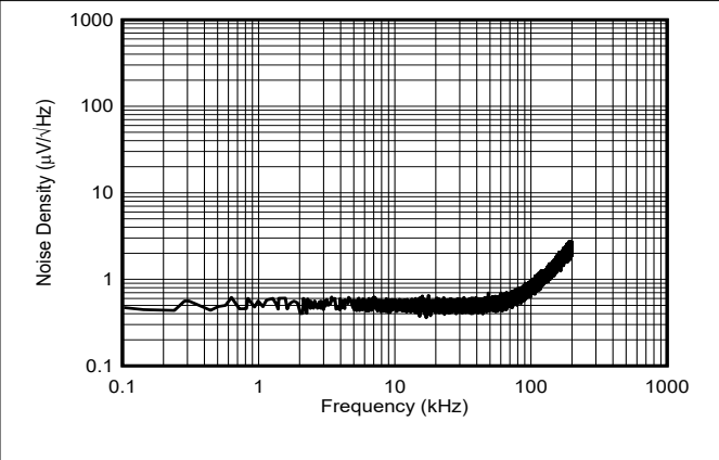
Figure 6-24. Input-Referred Noise Density vs Frequency
