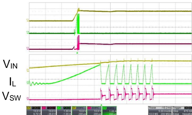
R_S Short ( V_{LED}=9\text{V} , R_S=0.3\Omega , L=47\mu\text{H} )
