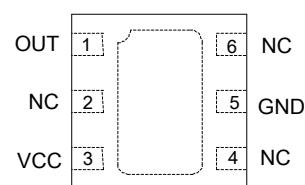
U-DFN2020-6 (Type C)
