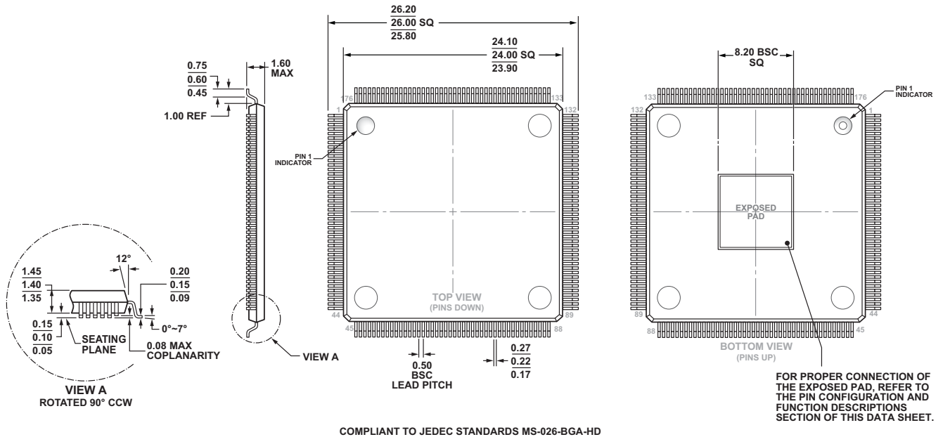
Figure 93. 176-Lead Low Profile Quad Flat Package, Exposed Pad [LQFP_EP]
