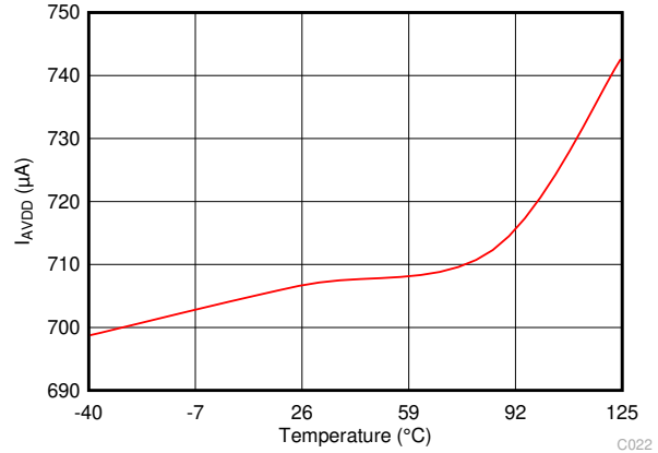
Figure 7-23. Analog Supply Current vs Temperature ( \text{OSC\_SEL} = 0 , \text{CLK\_DIV} = 0 ) in Turbo Comparator Mode C022
