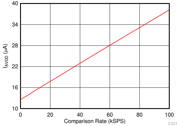
Figure 7-22. Analog Supply Current vs Comparison Rate ( \text{OSC\_SEL} = 1 ) in Turbo Comparator Mode C021
