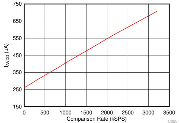
Figure 7-21. Analog Supply Current vs Comparison Rate ( \text{OSC\_SEL} = 0 ) in Turbo Comparator Mode C020
