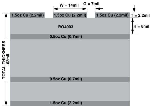
Figure 23. Evaluation Board Cross Sectional View
